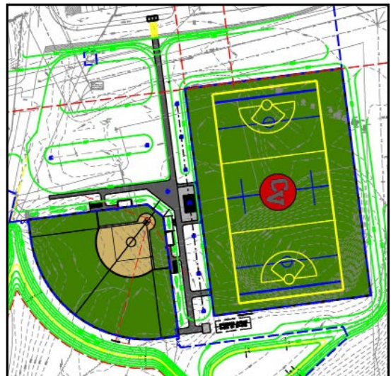
Middle/High School athletic field site plan.
